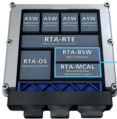
RTA-BSW includes everything customers need for functional safety-compliant applications.
