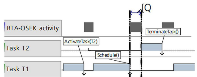
Figure 6 - Task chaining
